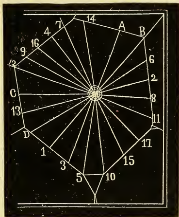
FIG. 73.—ALTERNATE APPPOSITION.
